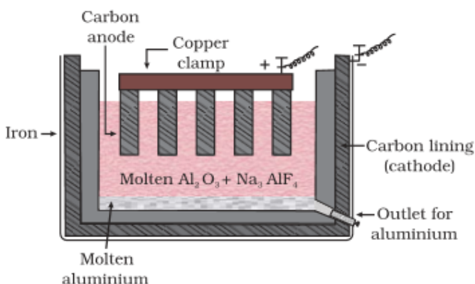
Fig: 3 Electrolytic Cell for Extraction of Aluminium, Source NCERT, Chemistry, PartI, XII
