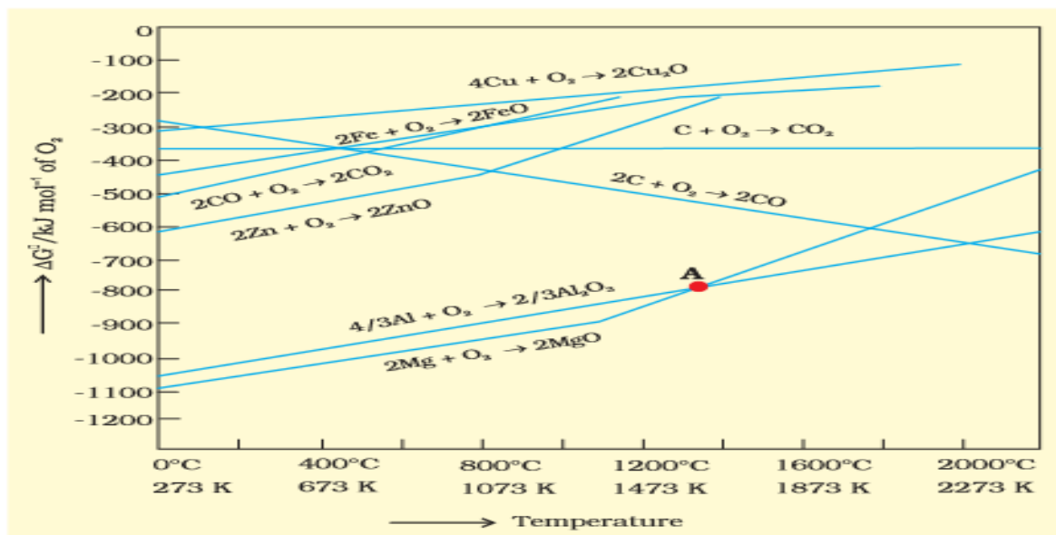
Figure 1: Gibbs energy ( \Delta G^0 ) vs T plots (schematic) for formation of some oxides:
