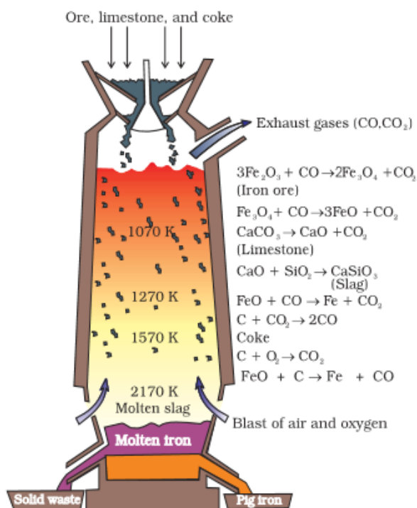
Figure:2: Blast furnace Source NCERT, Chemistry, Part I, XII
